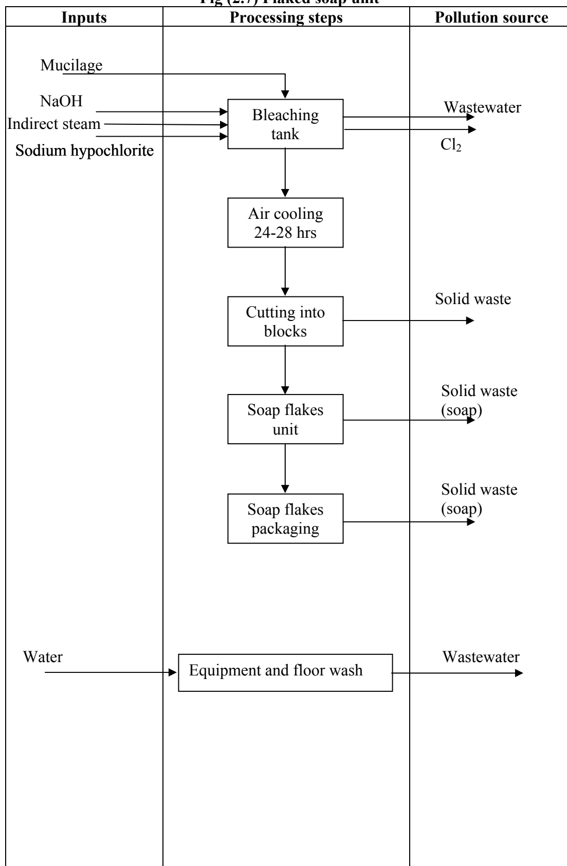
Fig (2.7) Flaked soap unit
