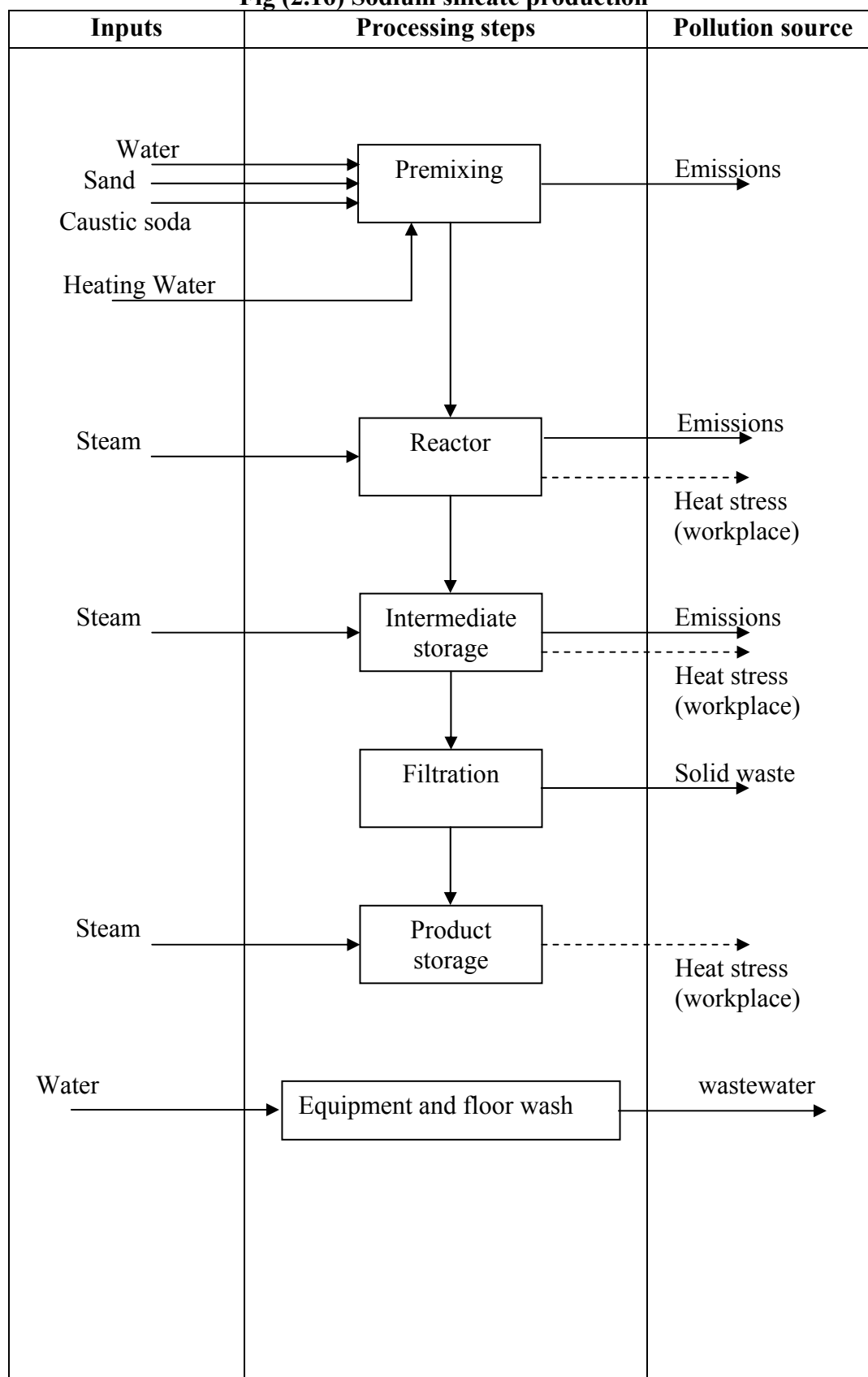
Fig (2.16) Sodium silicate production
