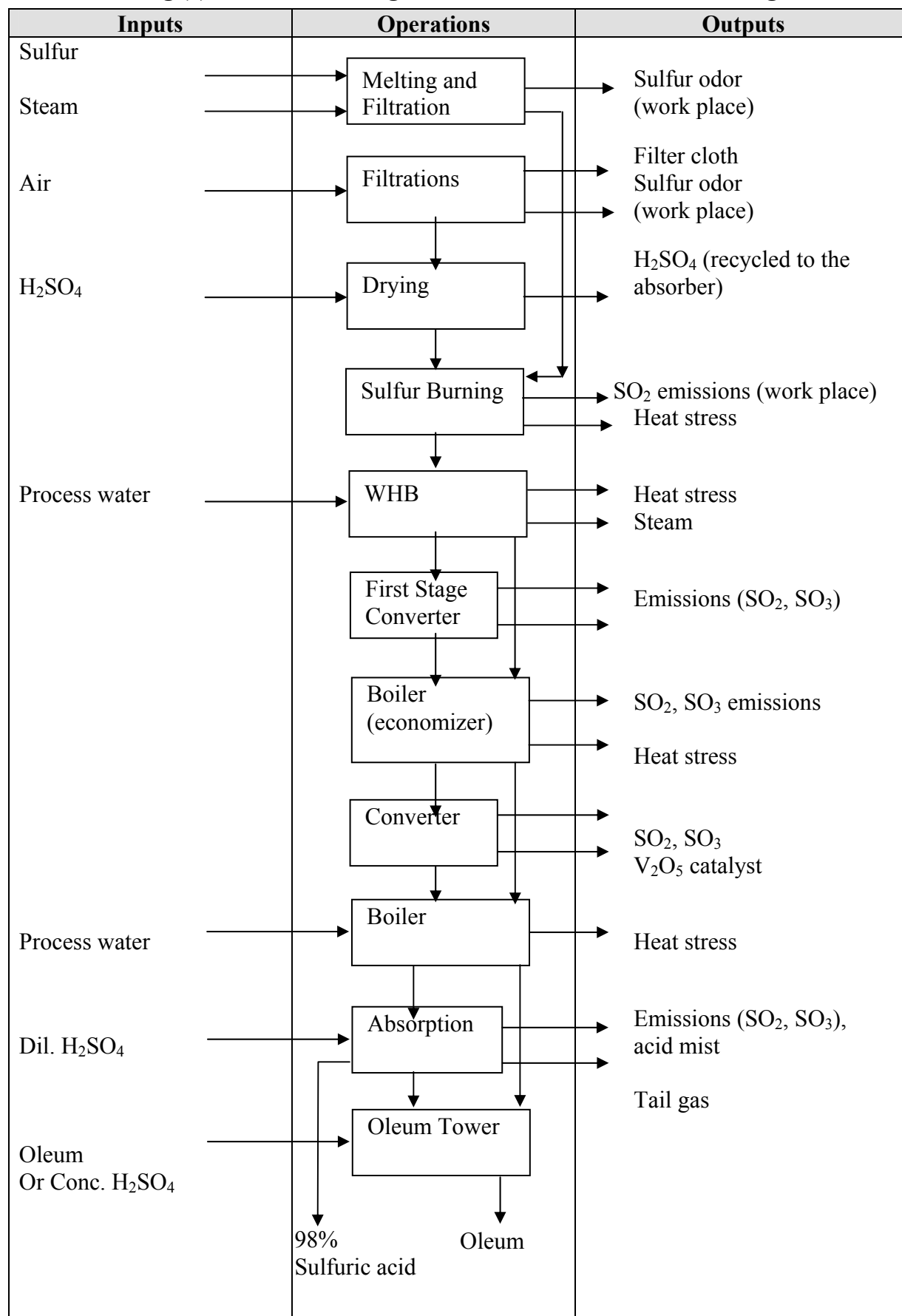
Fig (6) Process Flow Diagram for Sulfuric Acid Manufacturing
