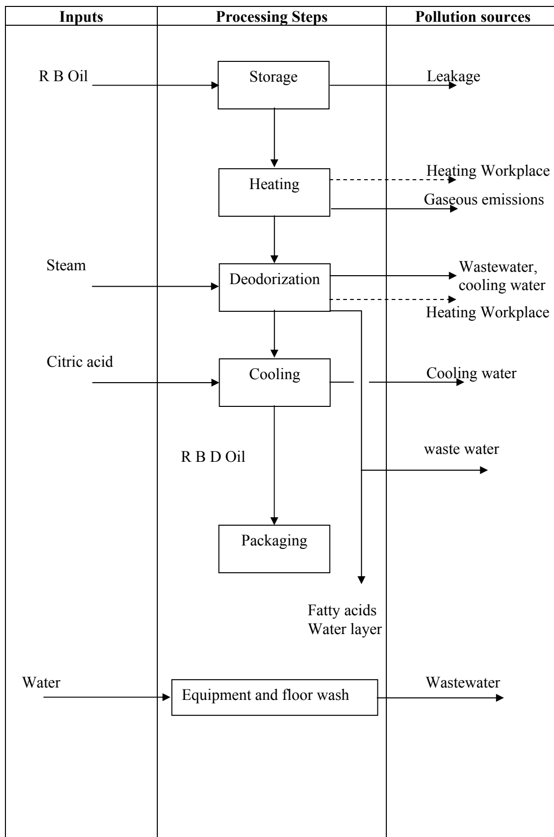
Fig (2.4) Deodorization
