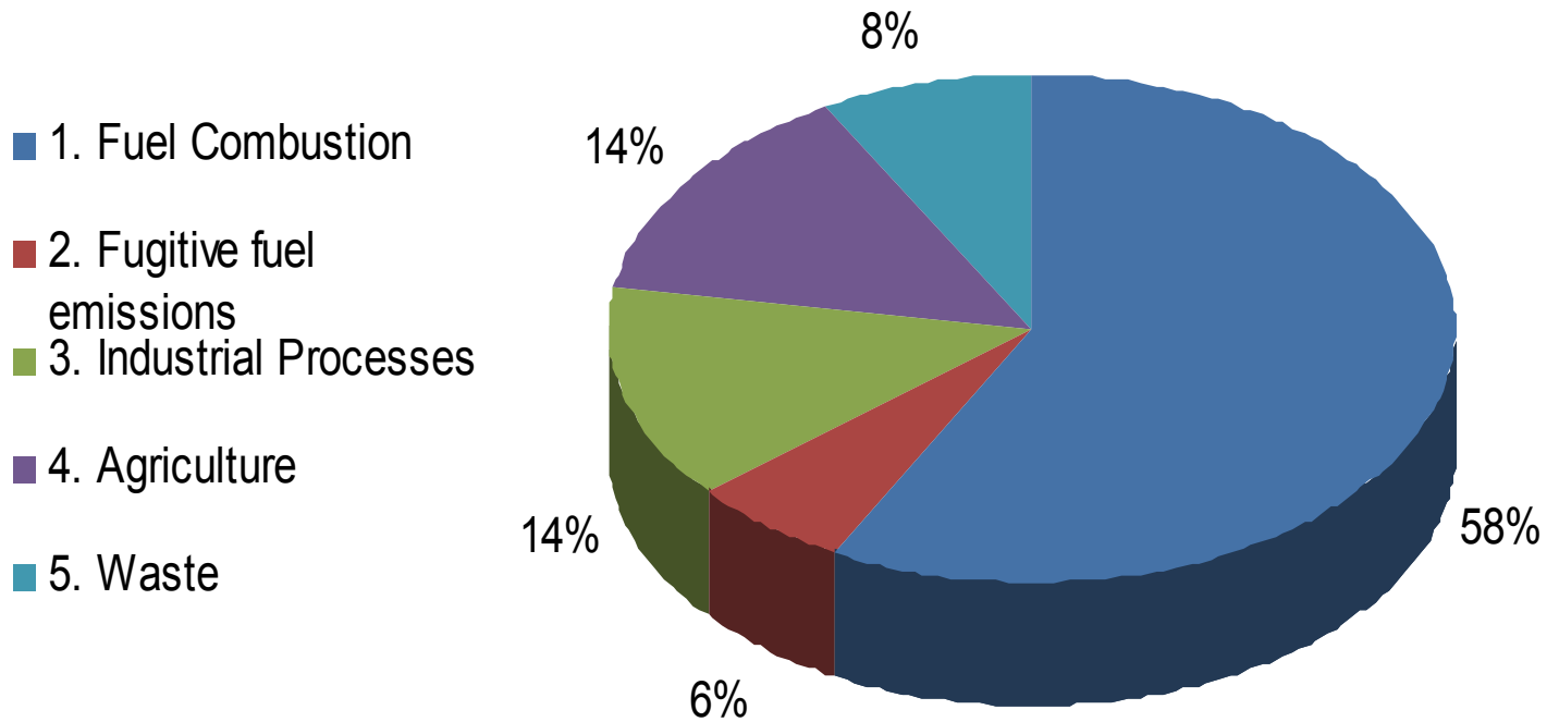
Fig (2): Emission by Sector, Million ton/year Percentage
