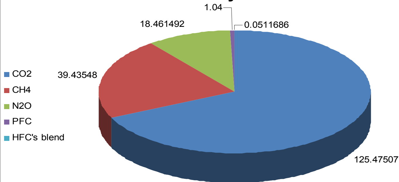
Fig(1): Egypt Emissions by Gas CO2e, million ton/ year
