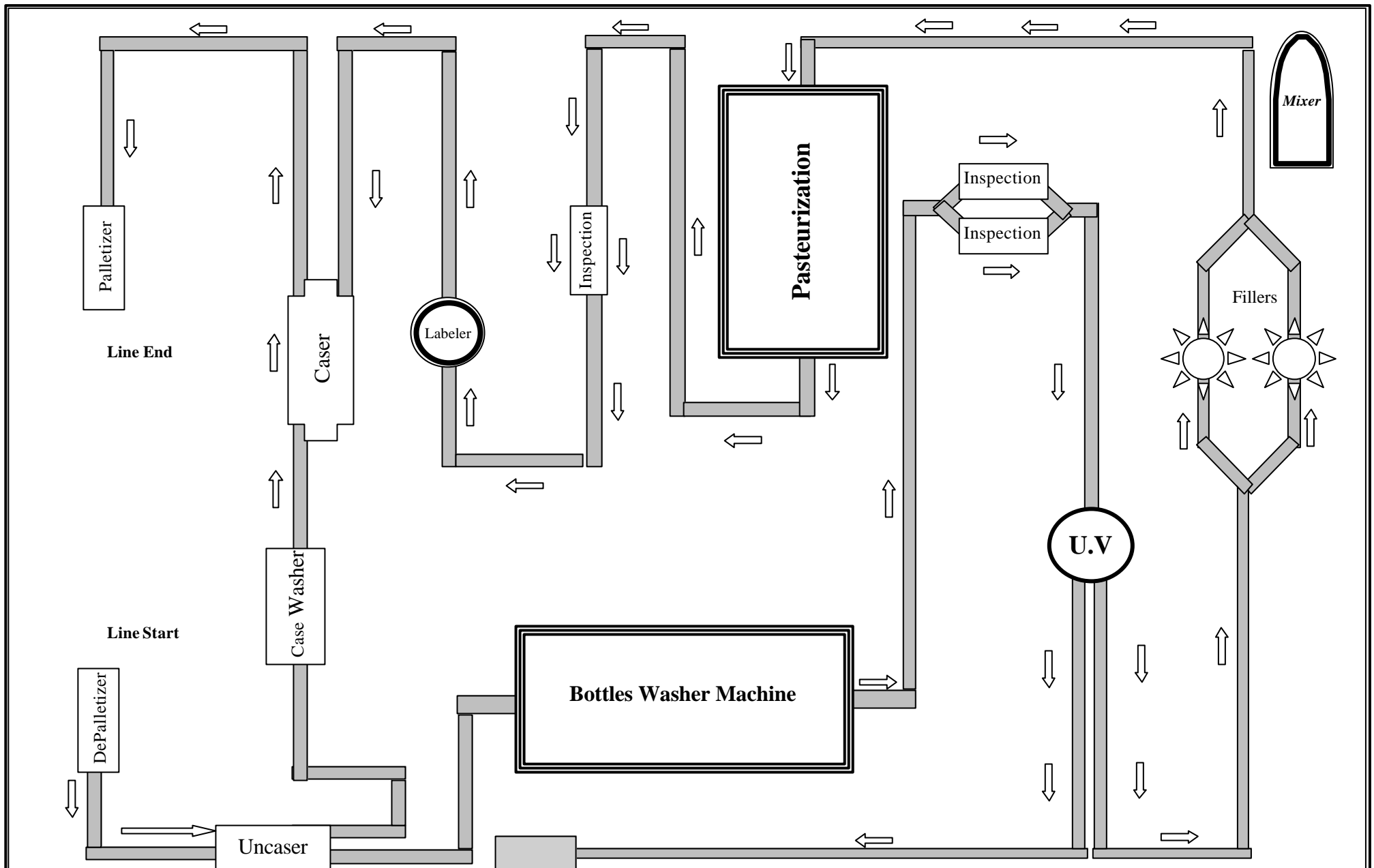
Figure (1): Typical Process Flow Diagram for Beverage and Soft Drink Industry U.V. =U.V Inspection Point
